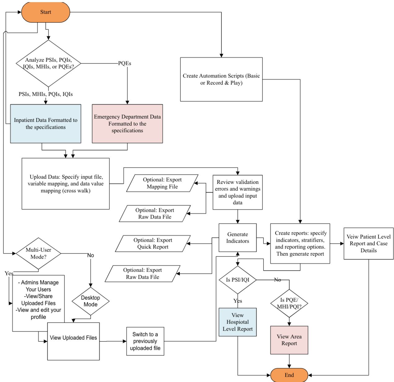
Figure 1. CloudQI Flowchart
